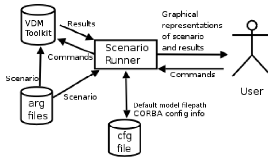
Figure 4.1: Context diagram for Validation GUI.
